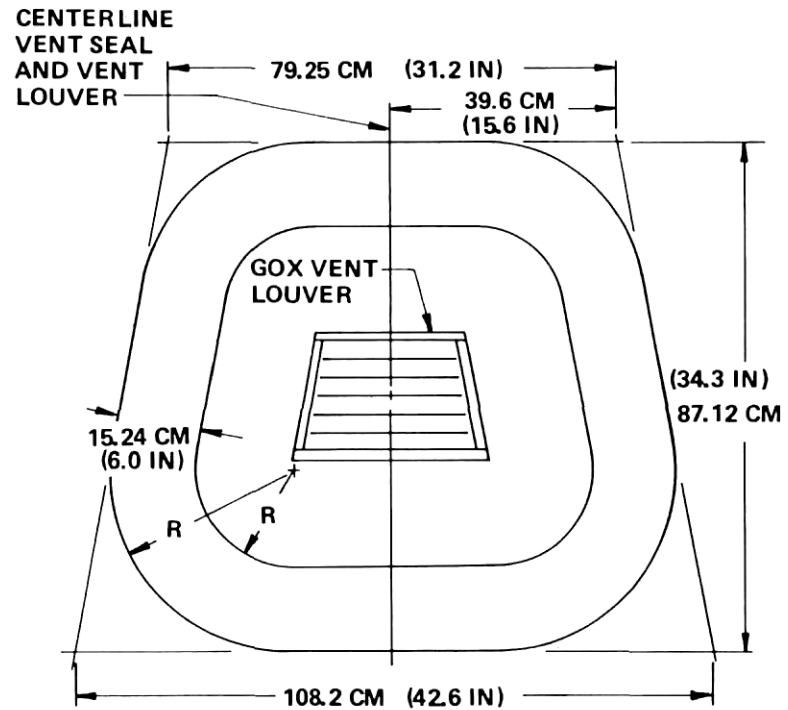
SECTION A-A SEAL FOOTPRINT
